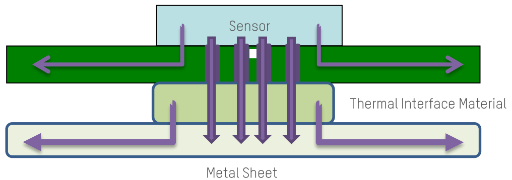
Figure 16 Non-Silicon Oil Heat Conduction and Dissipation
