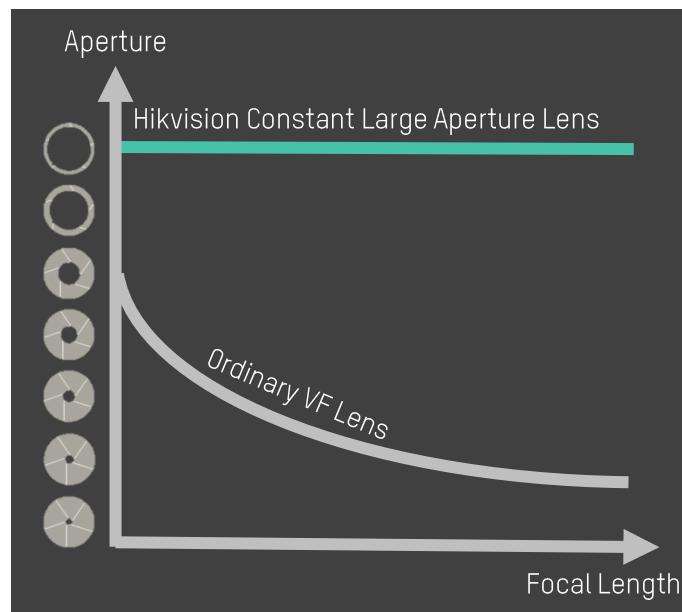
Figure 6 Constant Aperture
