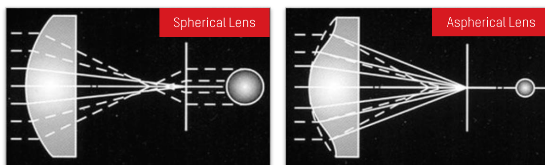
Figure 3 A Spherical Lens and an Aspherical Lens
