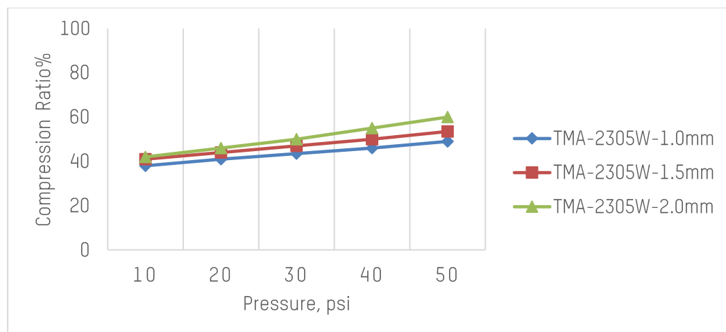
Figure 17 Compression Ratio Curve
